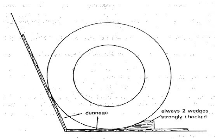
Figure 1 - Principle of dunnaging and wedging coils
