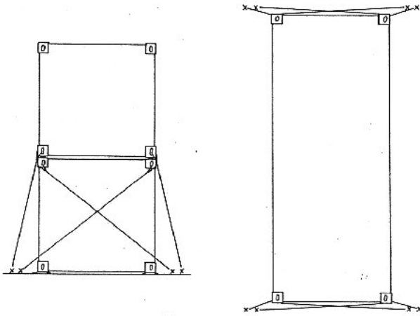
Figure 1 - Recommended methods of non-standardized securing of containers (cont.)
