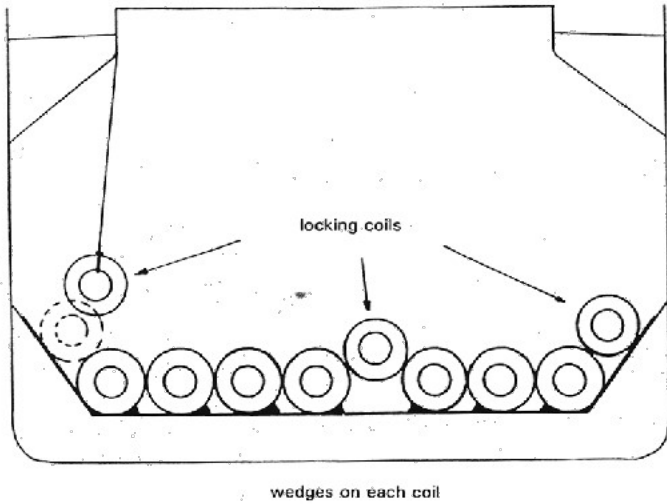
Figure 2- Inserting of locking coils
