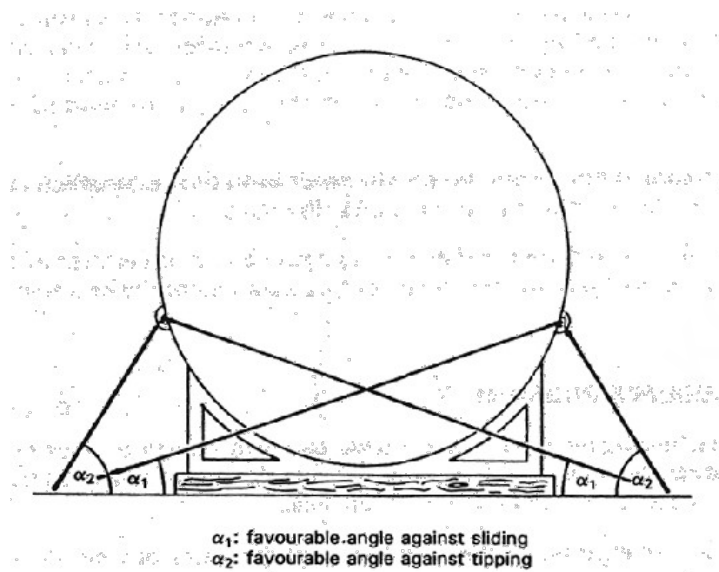
Figure 1 - Securing of portable tanks with favourable lashing angles
