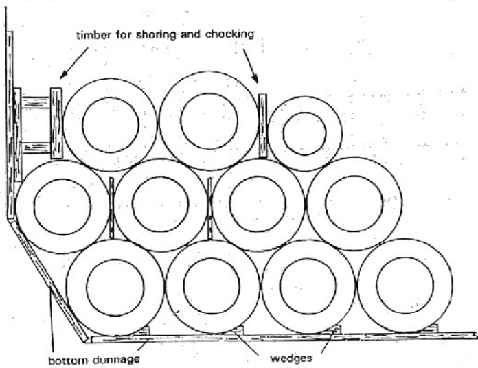
Figure 3- Shoring and chocking in voids between coils
