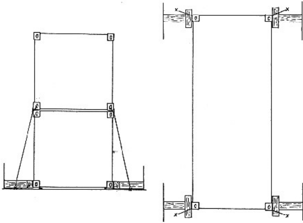
Figure 1- Recommended methods of non-standardized securing of containers
