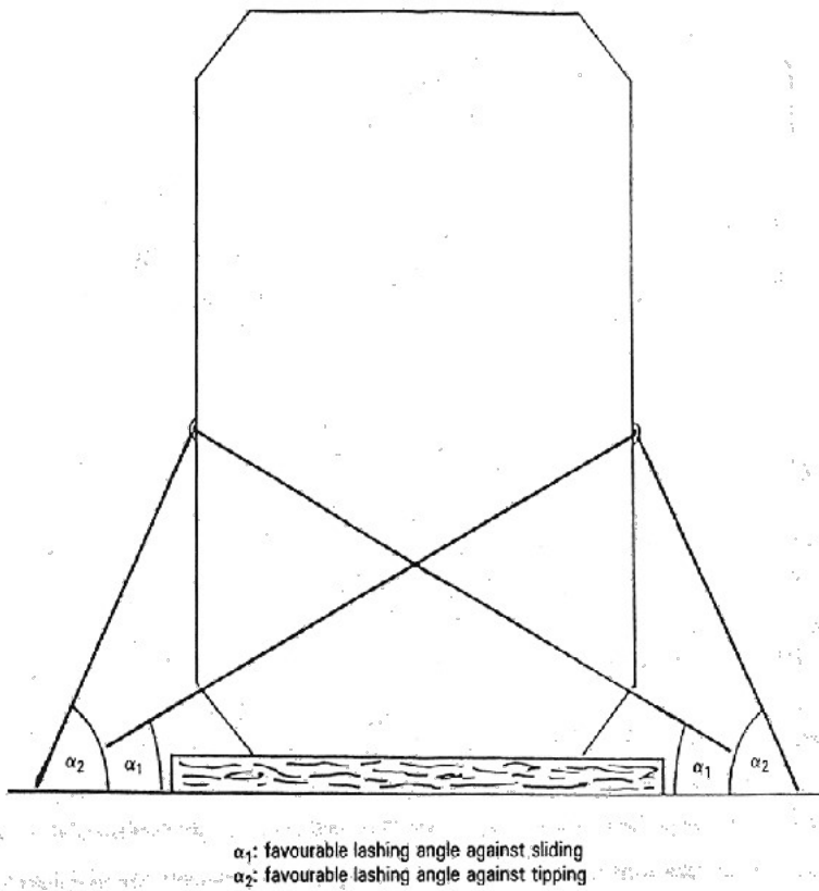
Figure 1- Principles of securing heavy items against sliding and tipping
